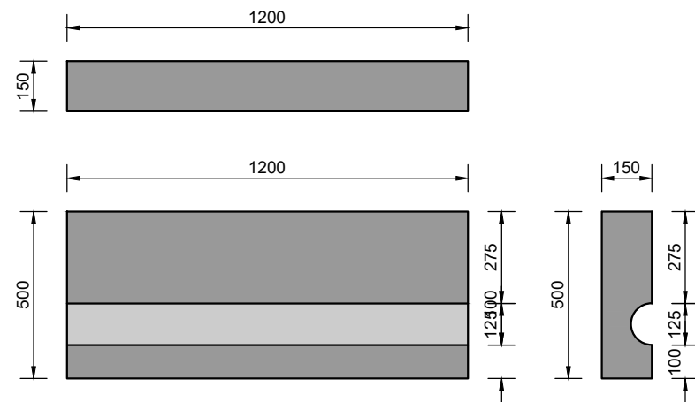
Detail 1: Rockflow WM2005 or WM2007 1200 x 500 x 150mm with 1 x 1/2 Ø125mm channel
