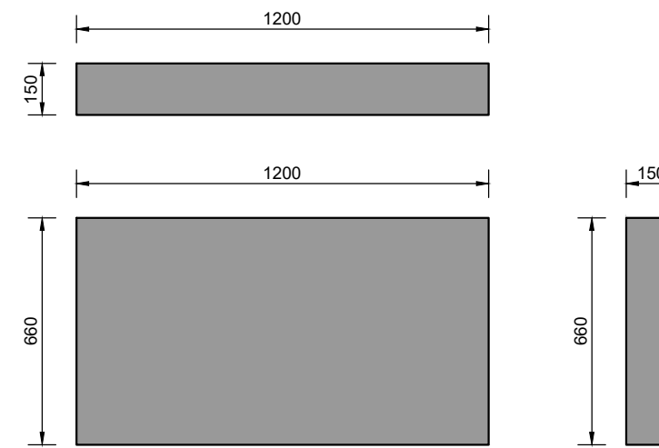
Detail 2: Rockflow WM2005 or WM2007 1200 x 660 x 150mm
