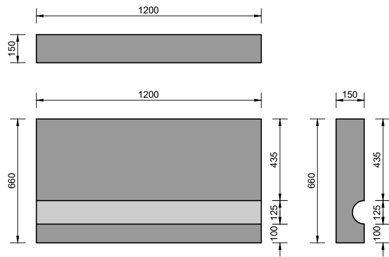
Detail 1: Rockflow WM2005 or WM2007 1200 x 660 x 150mm with 1 x 1/2 Ø125mm channel
