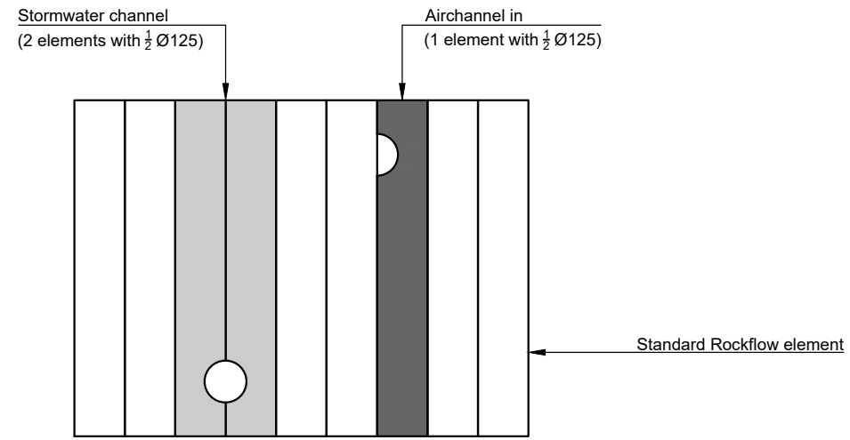
Cross section: Rockflow waterbuffer
